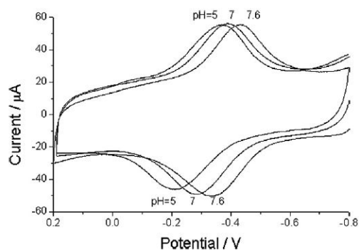
Fig. 6: Cyclic voltammetry study of Hb-CNT modified glassy carbon electrode at different pH values
