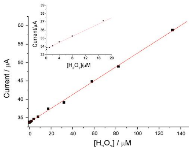
Fig. 7: Plot of the cathodic peak currents at Hb-CNT modified glassy carbon electrode in HAC-NaAc buffer solution versus H 2 O 2 concentration. The insert shows the plot at low H 2 O 2 concentration
