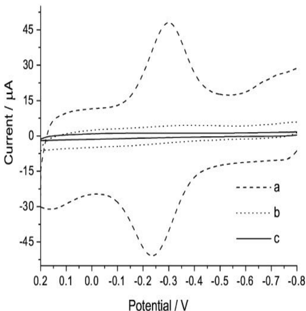
Fig. 3: Cyclic voltammetry study of Hb-CNT modified glassy carbon electrode in HAC-NaAc buffer solution (0.1 M, pH 5.0): (a) Hb-CNT assembled in the presence of EDC, (b) Hb-CNT assembled in the absence of EDC, and (c) bare GCE electrode. Scan rate 100 mV/s
