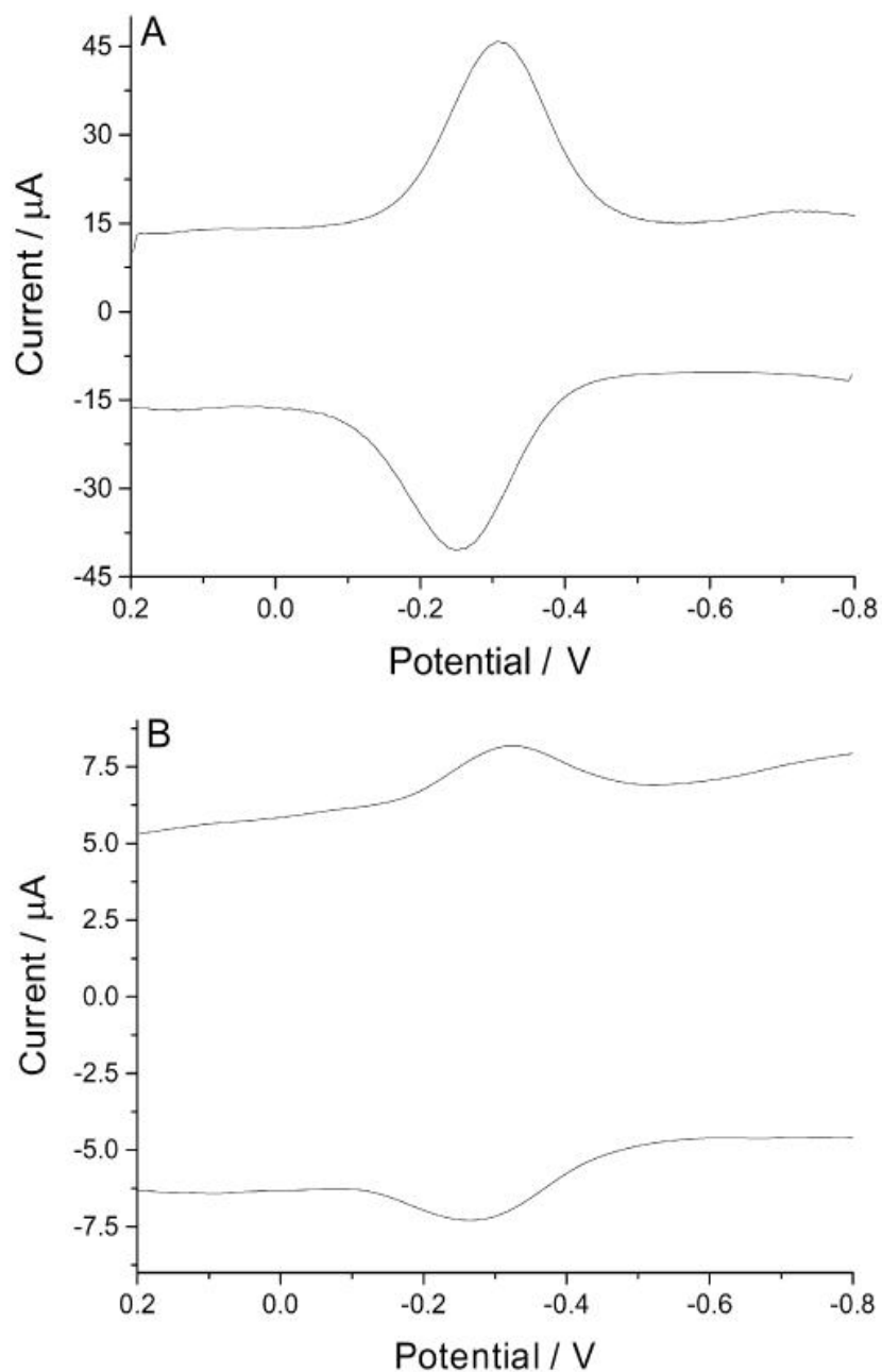
Fig. 4: Square wave voltammetry study of Hb-CNT modified glassy carbon electrode in HAC-NaAc buffer (0.1 M, pH 5.0): (A) Hb-CNT assembled in the presence of EDC, and (B) Hb-CNT assembled in the absence of EDC. Incr.4 mV, amplitude 25 mV, frequency 15 Hz
